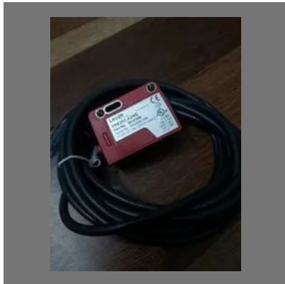
PRK25C.A2/6G - Polarized Retro-Reflective Photoelectric Sensor Part No.50141896
